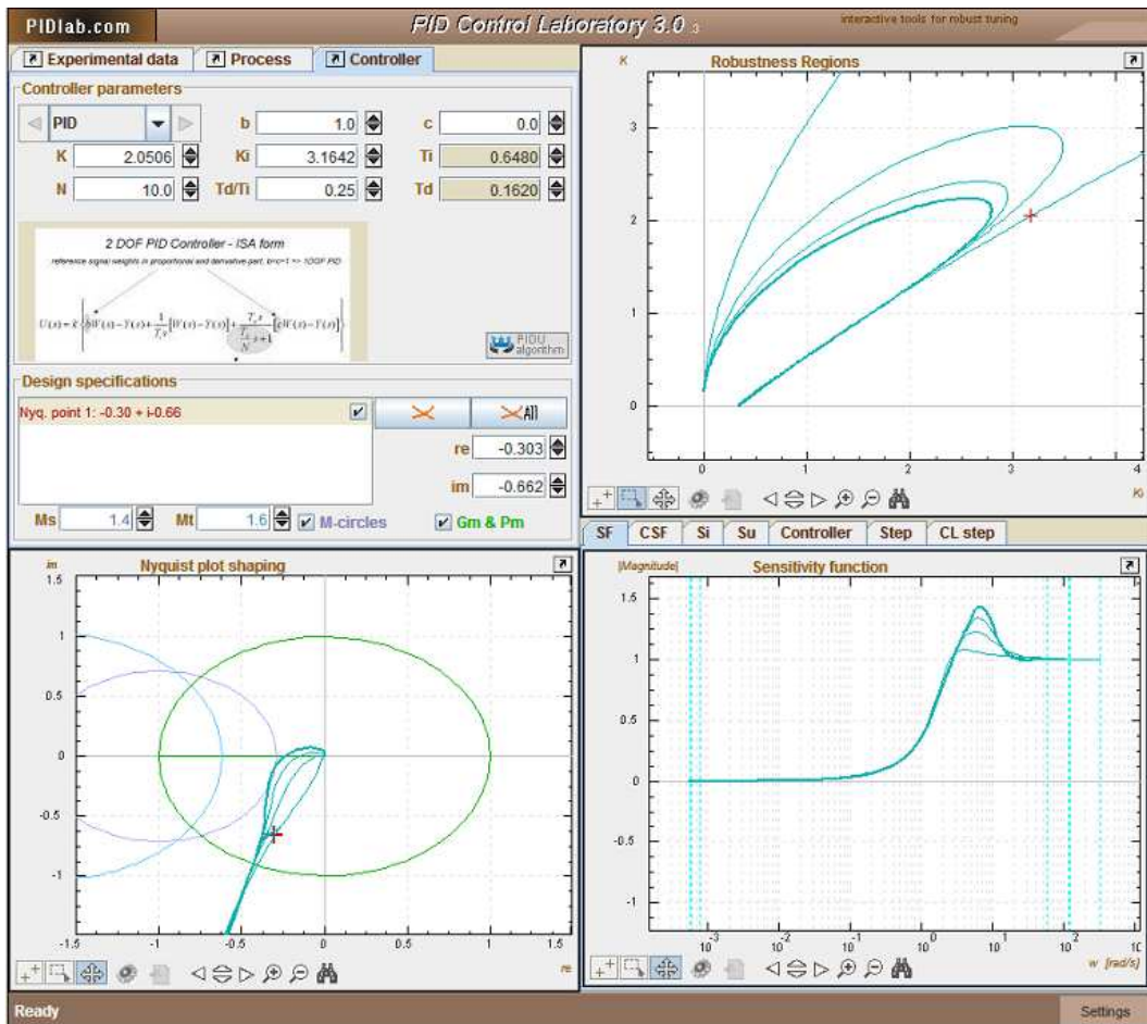
Fig. 4. Example of PIDlab applet for PID controller tuning. This applet adopts RexLib PIDU algorithm which was transformed manually into Java.
