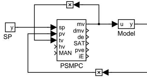
Fig. 5. Example of PSMPC demo drawn using RexLib blocks in Simulink editor.
